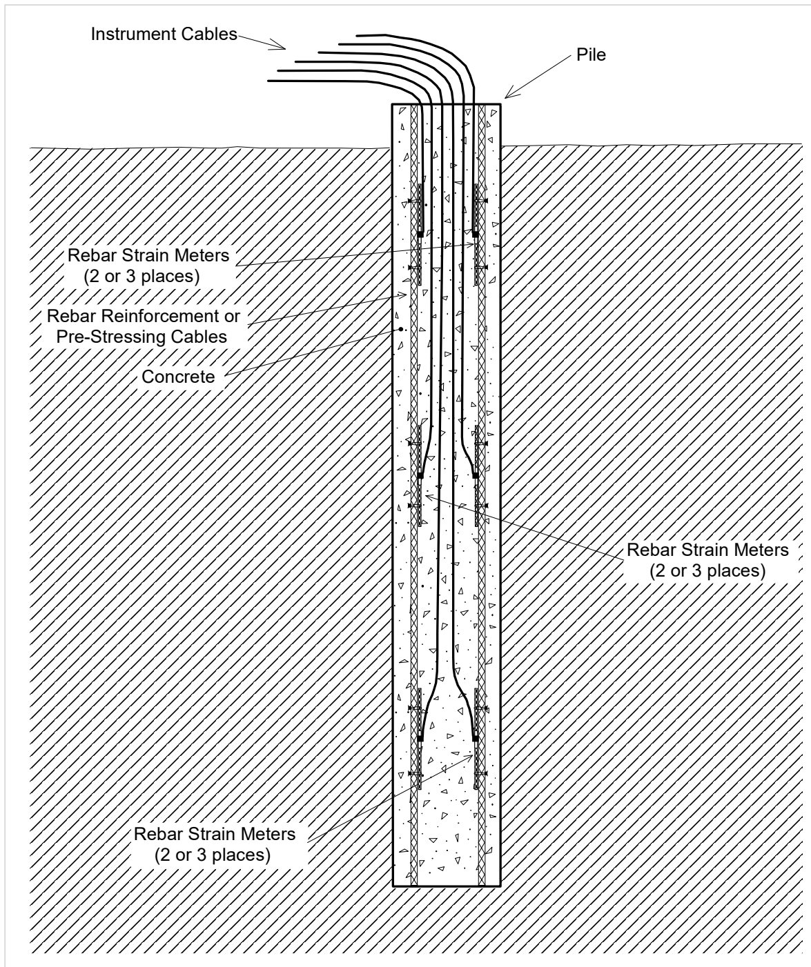
Figure 4 – ST5 - 12 “Sister Bar” Installation
