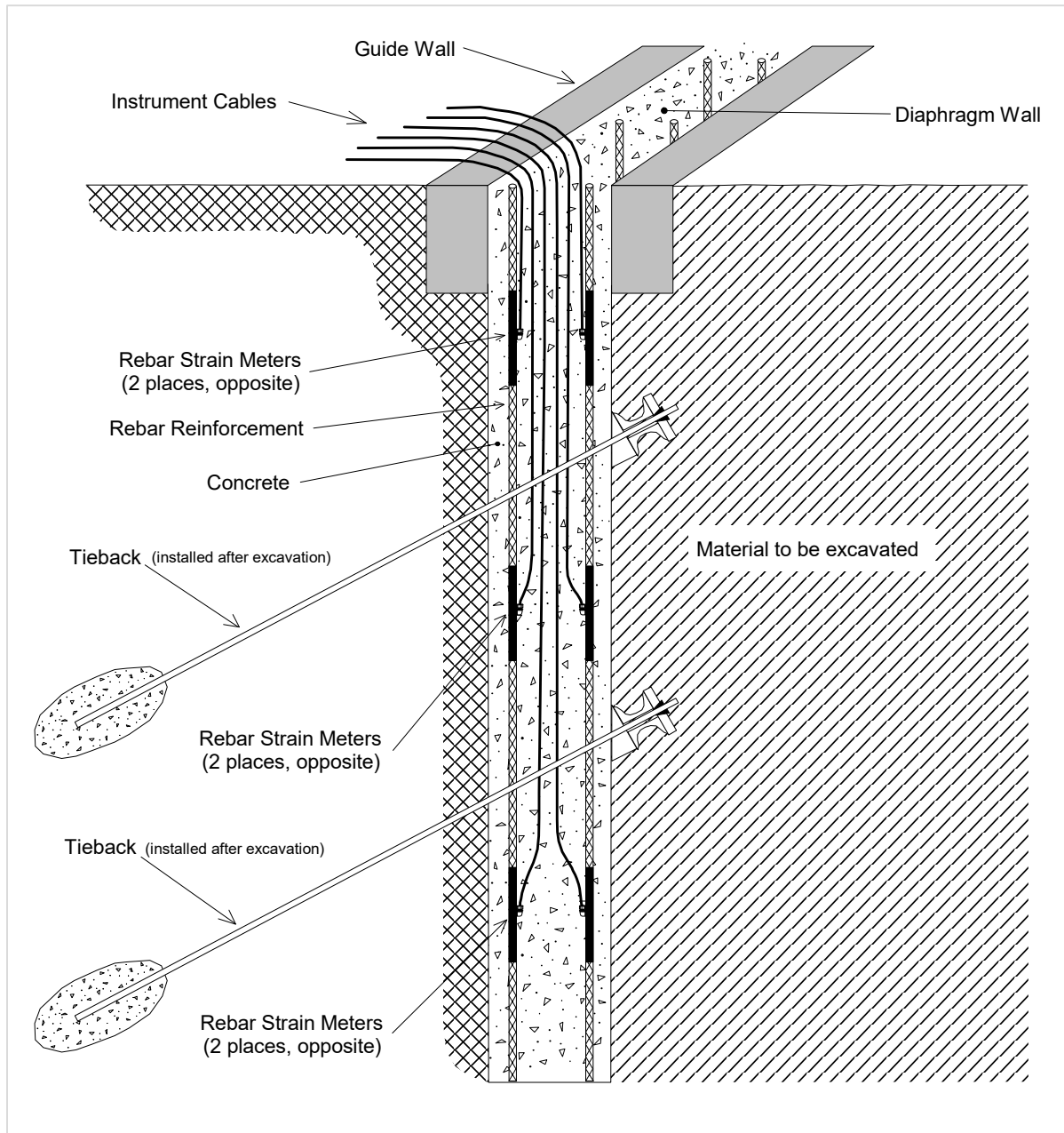
Figure 3 - Model ST5 – 16 to 40 Installation
