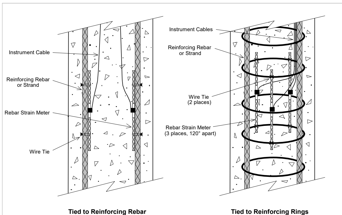
Figure 5 - Model ST5 - 12 "Sister Bar" Installation Detail
